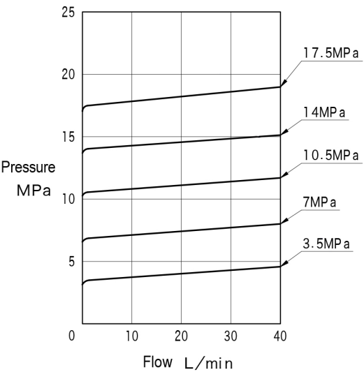
Flow-Pressure Characteristics
