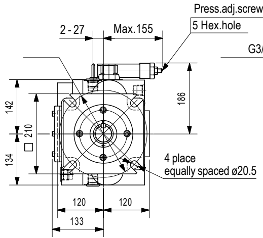
FOOT MOUNT
