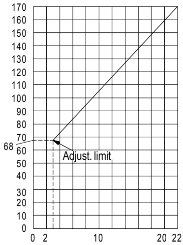
PH170 SERIES
