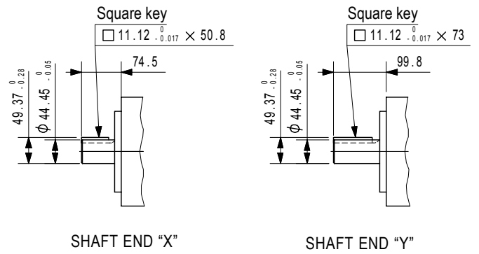
SHAFT END
